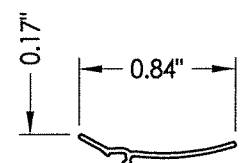
2 GLAZING BEAD
