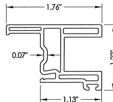
8 STILE/RAIL
