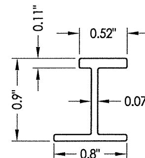
9 REINFORCEMENT
