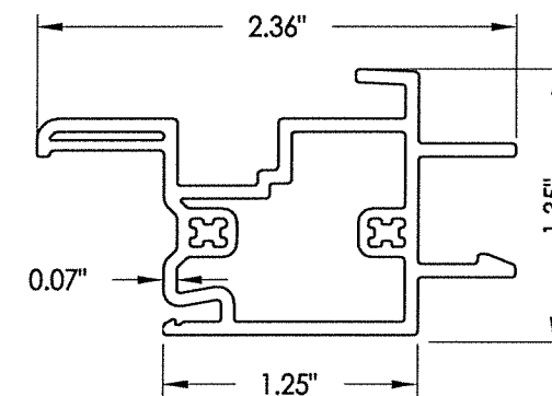
6 MEETING RAIL
