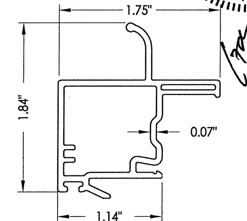
7 LOCK RAIL
